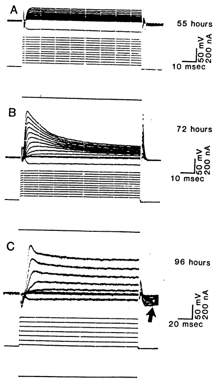
Fig. 1. Voltage clamp experiments showing DLM membrane currents at different stages of pupal development. (A to C) Hours are timed from puparium formation; current is shown in the upper traces, voltage in the lower traces. Outward current is in the upward direction. Holding potentials in (A) and (B), -60 mV; in (C), -80 mV. Because of the high capacitance of these fibers (approximately 0.02 \mu\text{F} ) and limitations of the voltage clamp equipment, accurate current readings cannot be made until approximately 3 msec after the command pulse is initiated. The initial rising slope of current is therefore due to charging time rather than to the opening of a current channel. See text for explanation of arrow. (D and E) Current-voltage relationships for DLM fibers; the early peak current component at 72 and 96 hours is shown in (D), and the steady-state current at 72 and 96 hours is shown in (E). Current in (E) is measured 200 msec after command pulses are applied.
